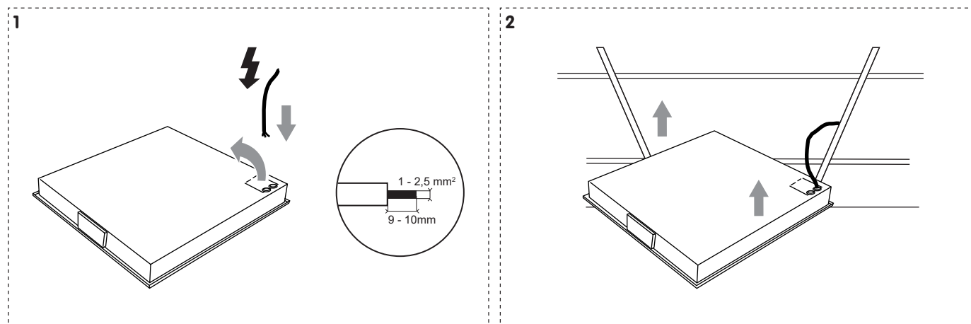
Montaje en techo modular perfil visto. Modular ceiling with exposed T-bar mounting.
